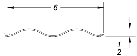
SINGLE CORRUGATED PANEL
